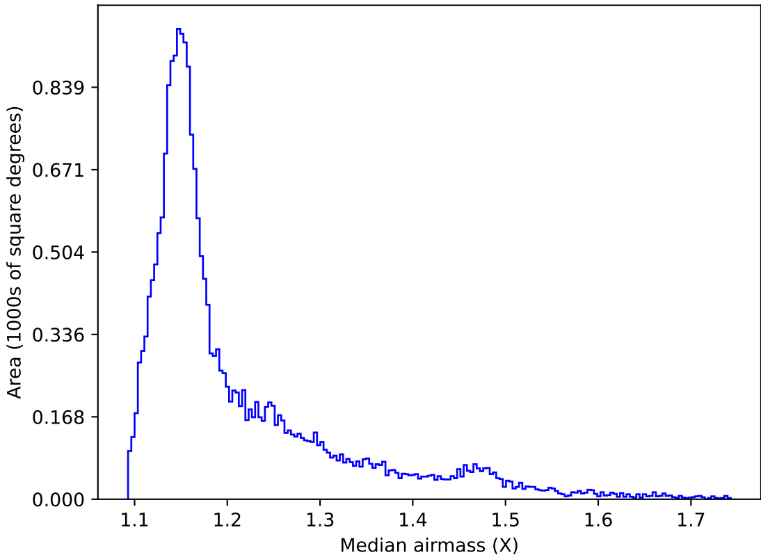
too_elab_r64_d2_giz_v3.4_10yrs All sky y band: Median airmass
