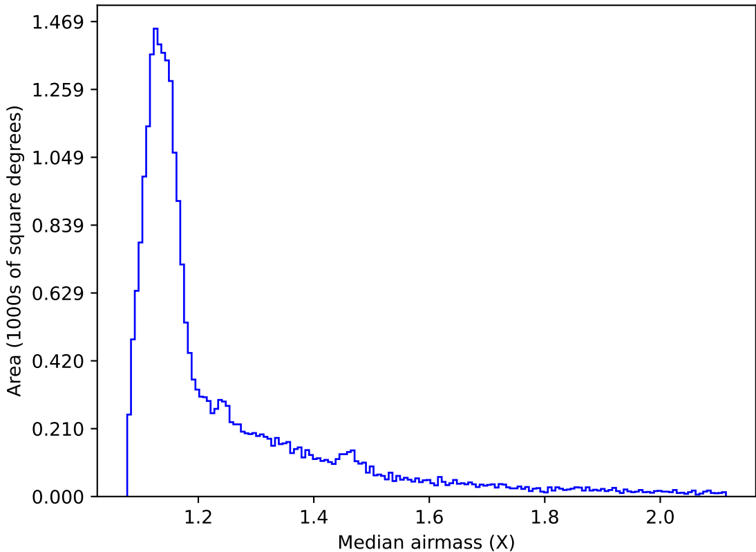
too_elab_r64_d2_giz_v3.4_10yrs All sky r band: Median airmass
