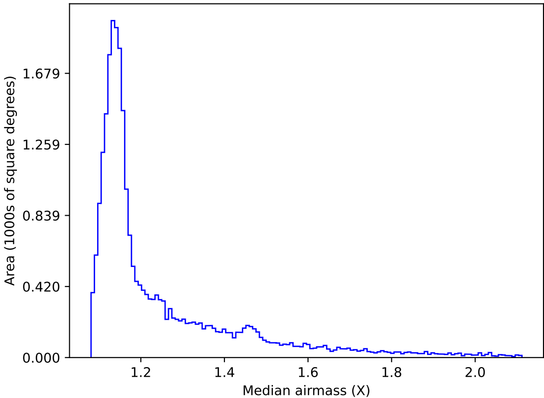
too_elab_r64_d2_giz_v3.4_10yrs All sky i band: Median airmass
