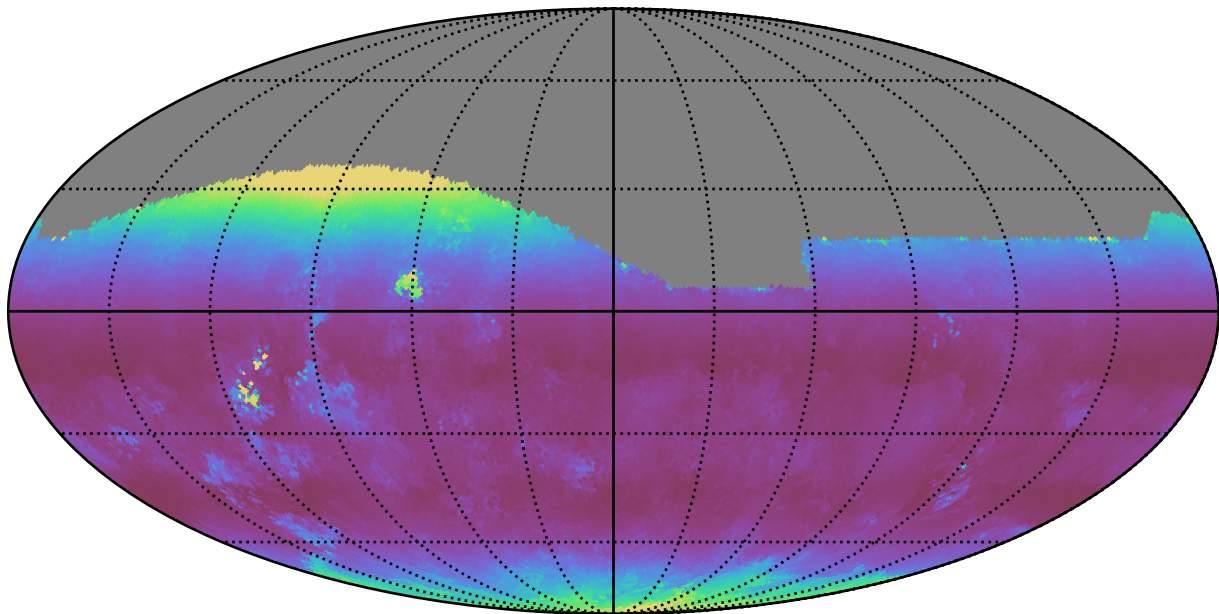
too_elab_r64_d2_giz_v3.4_10yrs All sky g band: Median airmass
