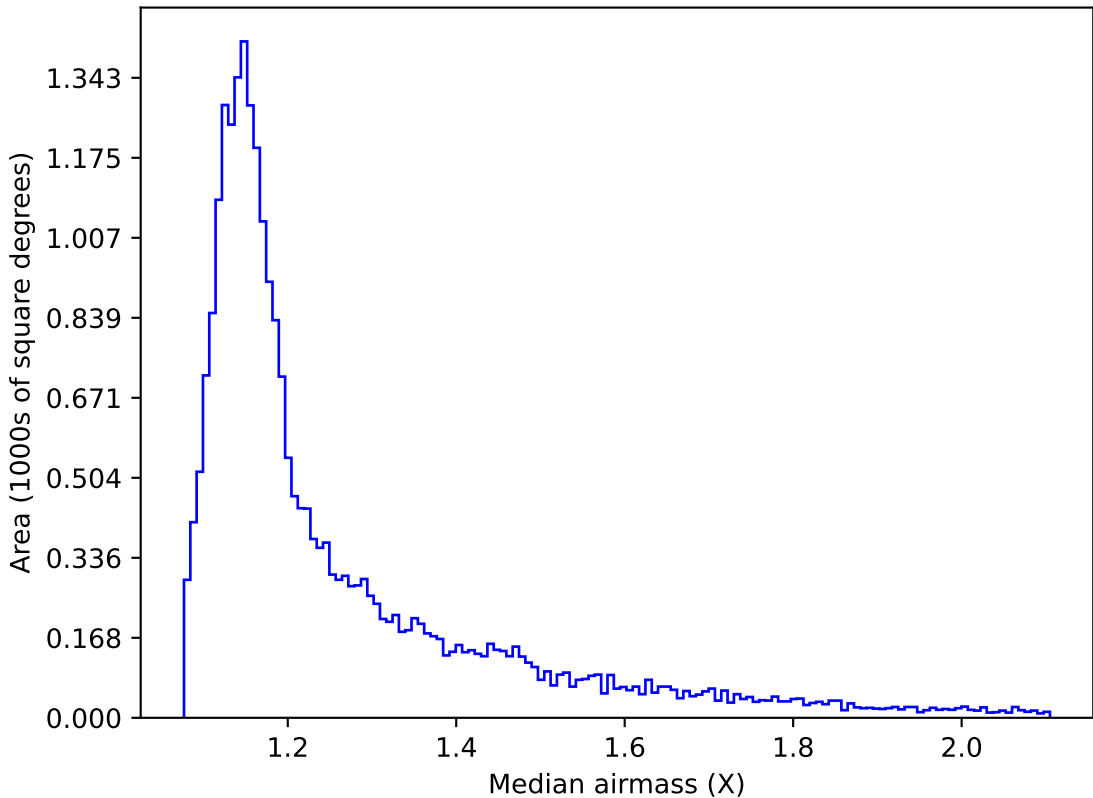
too_elab_r64_d2_giz_v3.4_10yrs All sky g band: Median airmass
