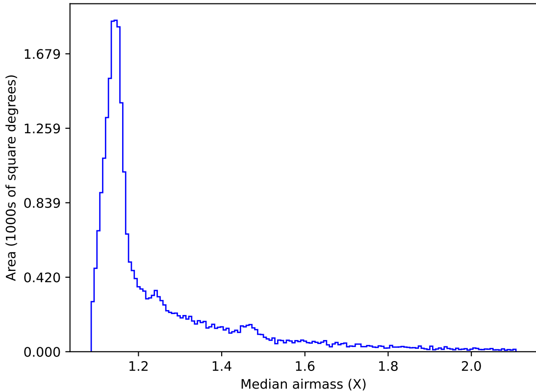
too_elab_r64_d2_giz_v3.4_10yrs All sky all bands: Median airmass
