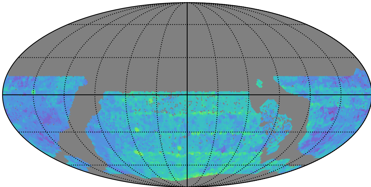
too_elab_r64_d2_giz_v3.4_10yrs WFD y band: Median Season Length
