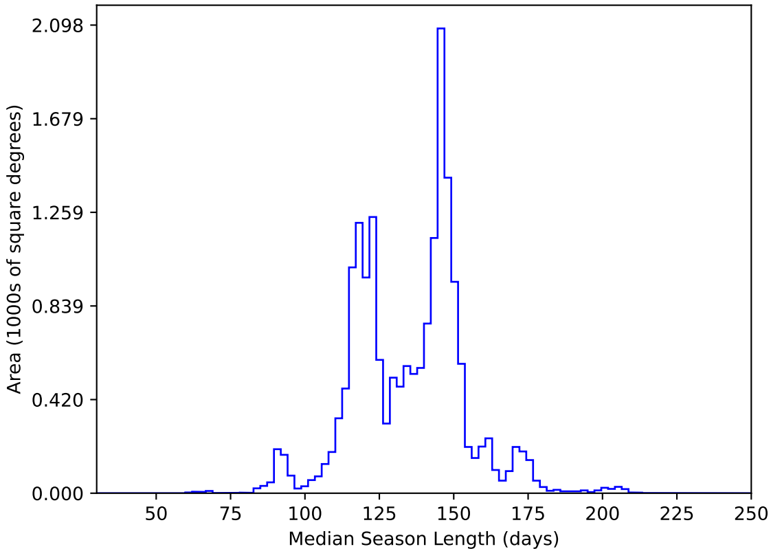
too_elab_r64_d2_giz_v3.4_10yrs WFD y band: Median Season Length
