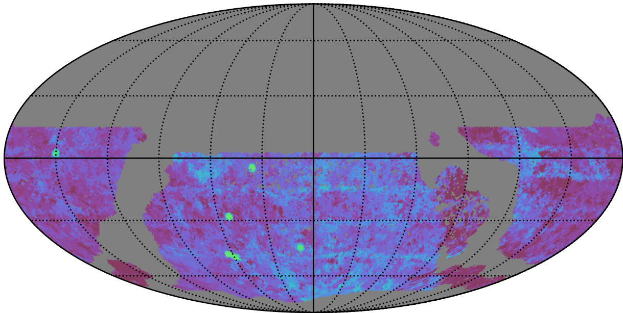
too_elab_r64_d2_giz_v3.4_10yrs WFD u band: Median Season Length
