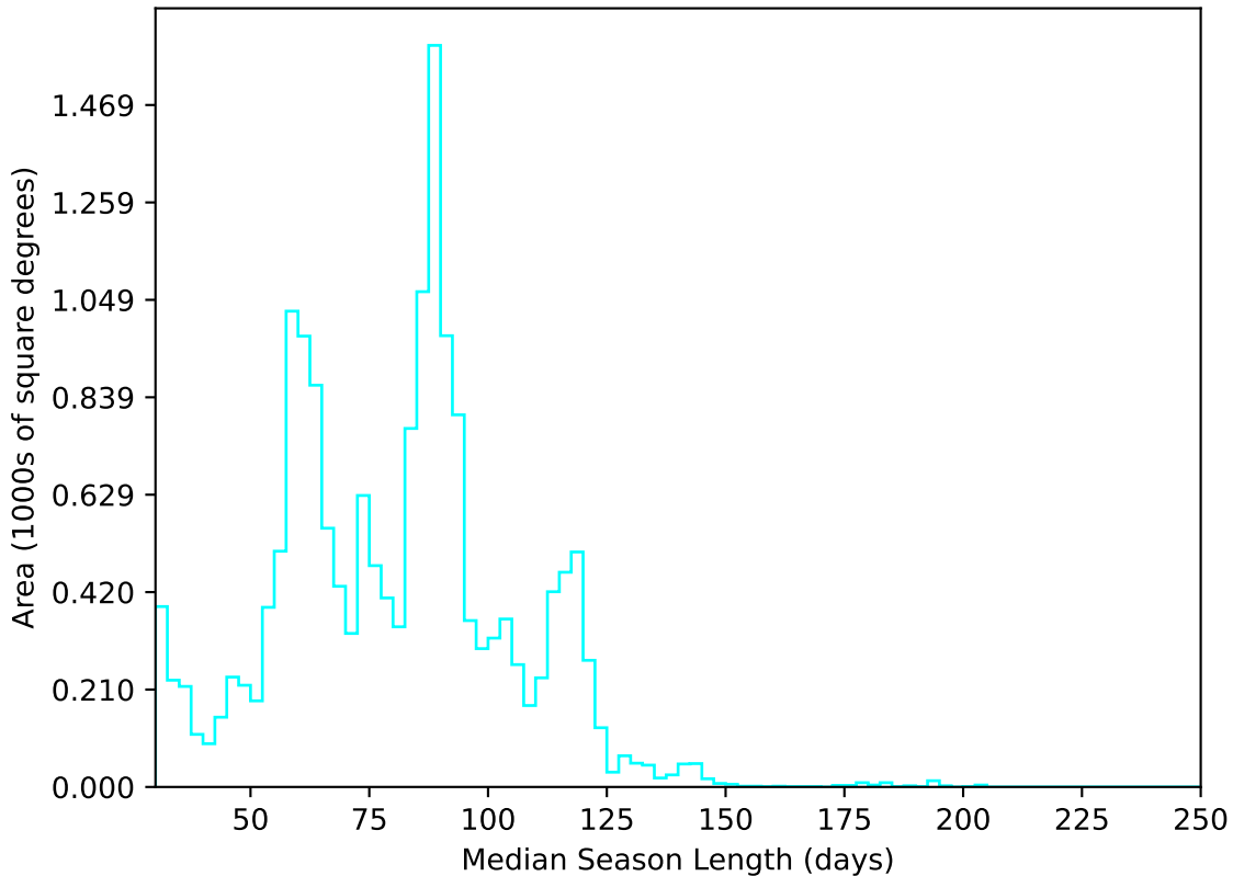
too_elab_r64_d2_giz_v3.4_10yrs WFD u band: Median Season Length
