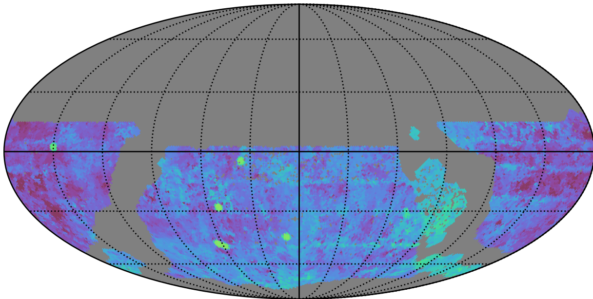
too_elab_r64_d2_giz_v3.4_10yrs WFD g band: Median Season Length
