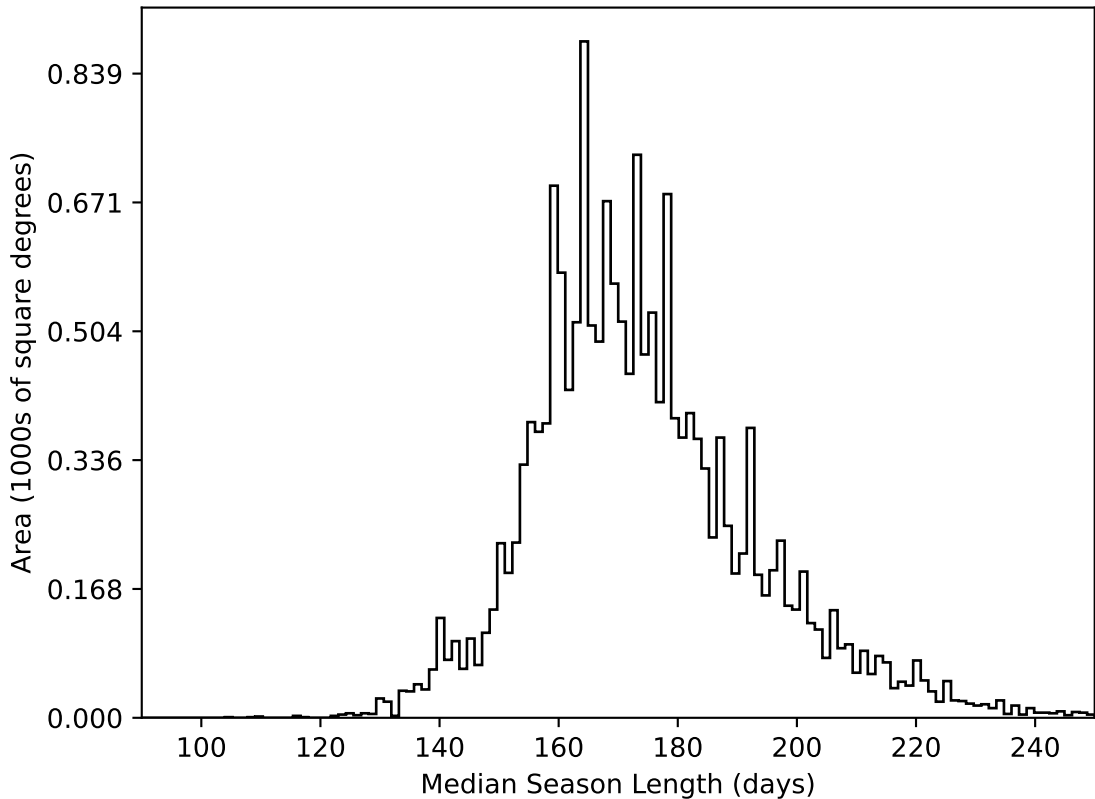
too_elab_r64_d2_giz_v3.4_10yrs WFD all bands: Median Season Length
