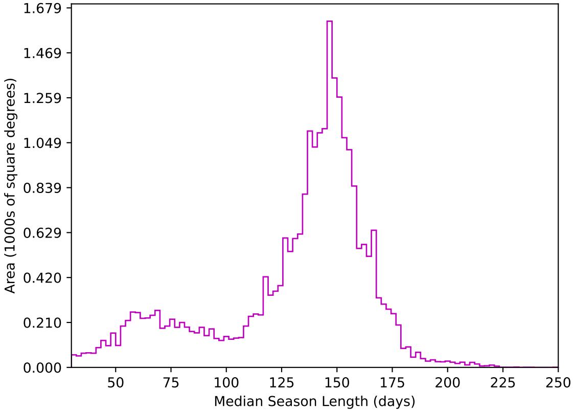
too_elab_r64_d2_giz_v3.4_10yrs All sky z band: Median Season Length
