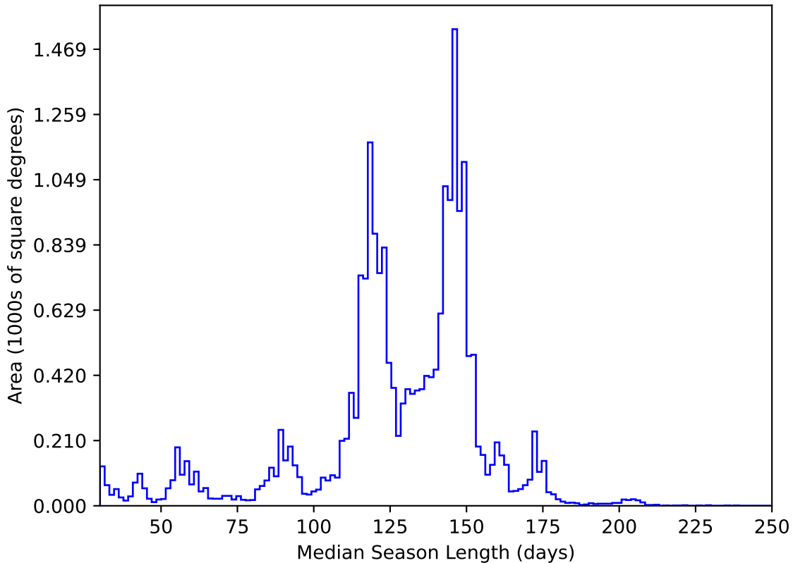
too_elab_r64_d2_giz_v3.4_10yrs All sky y band: Median Season Length
