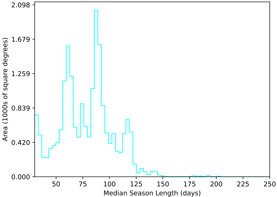
too_elab_r64_d2_giz_v3.4_10yrs All sky u band: Median Season Length
