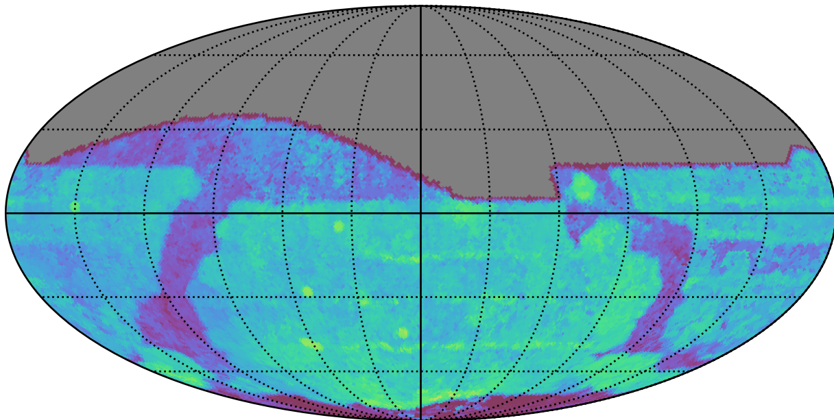
too_elab_r64_d2_giz_v3.4_10yrs All sky i band: Median Season Length
