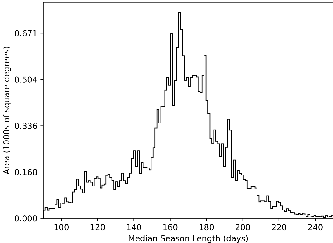
too_elab_r64_d2_giz_v3.4_10yrs All sky all bands: Median Season Length
