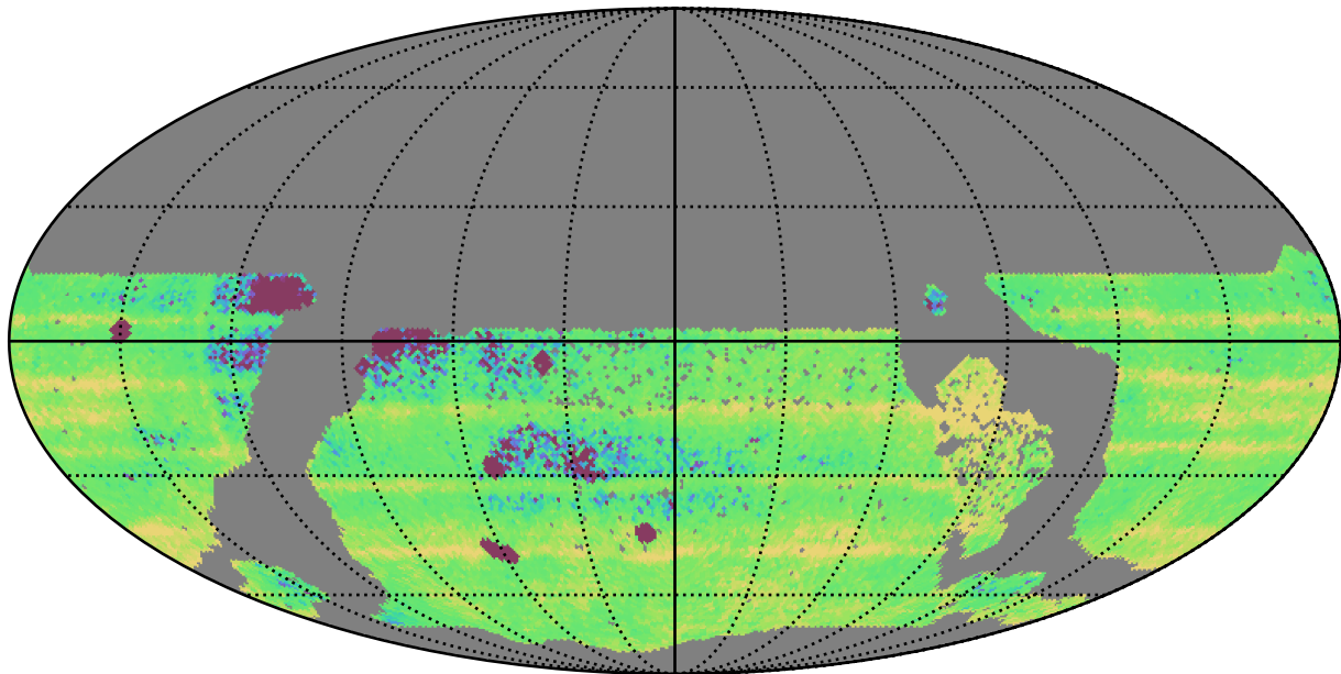
too_elab_r64_d2_giz_v3.4_10yrs WFD: Median Intra-Night Gap
