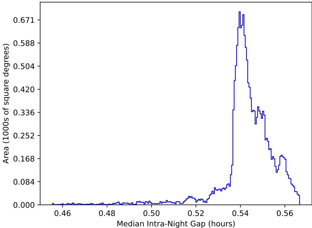
too_elab_r64_d2_giz_v3.4_10yrs WFD: Median Intra-Night Gap
