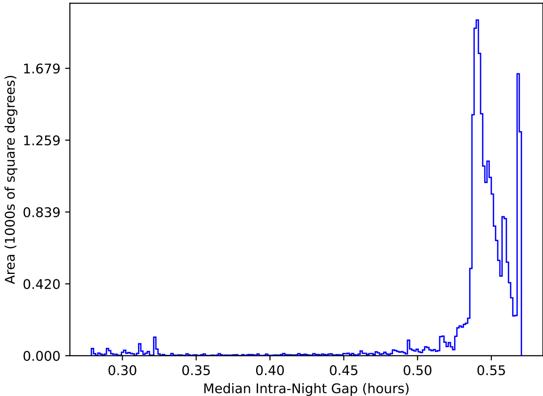
too_elab_r64_d2_giz_v3.4_10yrs All sky: Median Intra-Night Gap
