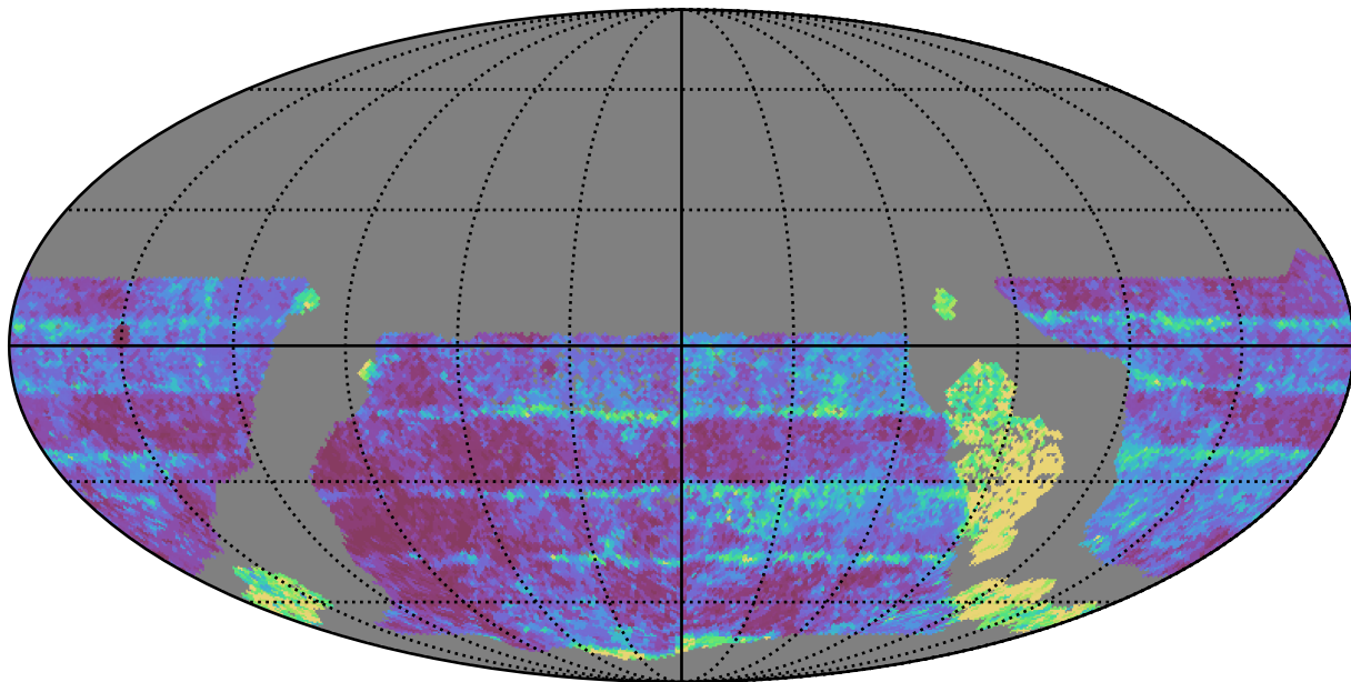
too_elab_r64_d2_giz_v3.4_10yrs WFD z band: Median Inter-Night Gap
