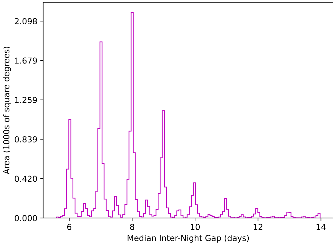
too_elab_r64_d2_giz_v3.4_10yrs WFD z band: Median Inter-Night Gap
