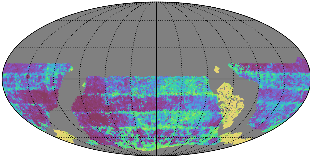
too_elab_r64_d2_giz_v3.4_10yrs WFD y band: Median Inter-Night Gap
