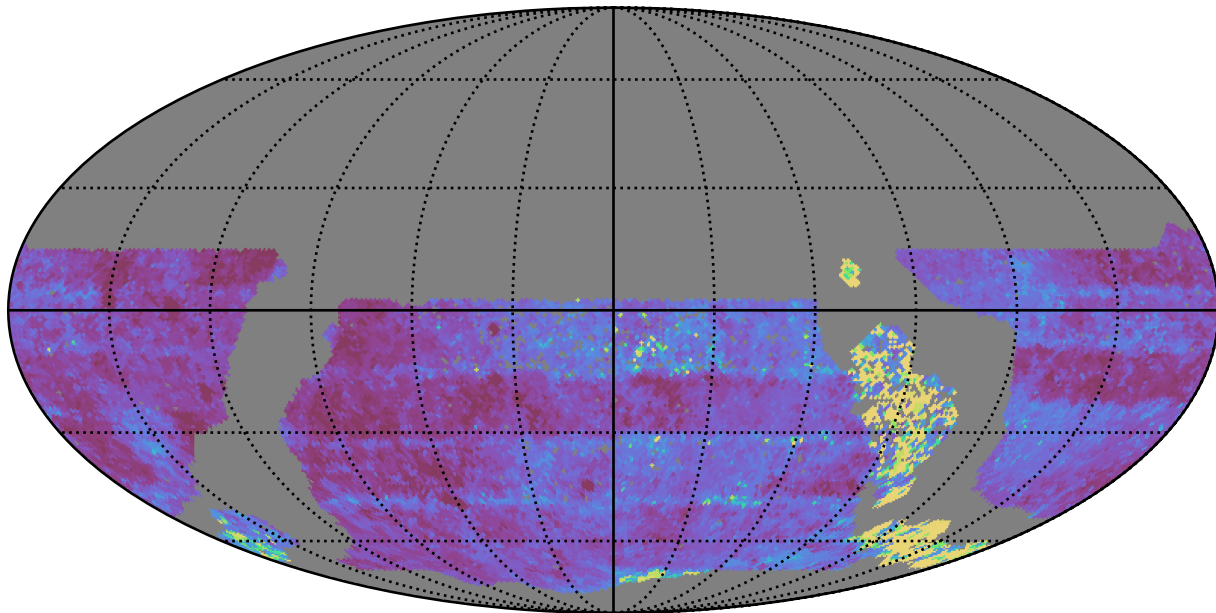
too_elab_r64_d2_giz_v3.4_10yrs WFD u band: Median Inter-Night Gap
