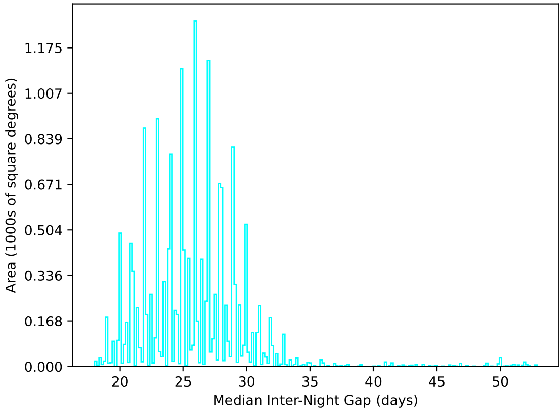
too_elab_r64_d2_giz_v3.4_10yrs WFD u band: Median Inter-Night Gap
