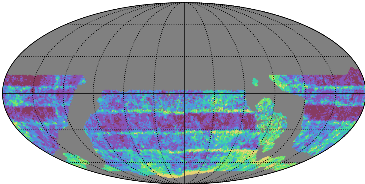
too_elab_r64_d2_giz_v3.4_10yrs WFD r band: Median Inter-Night Gap
