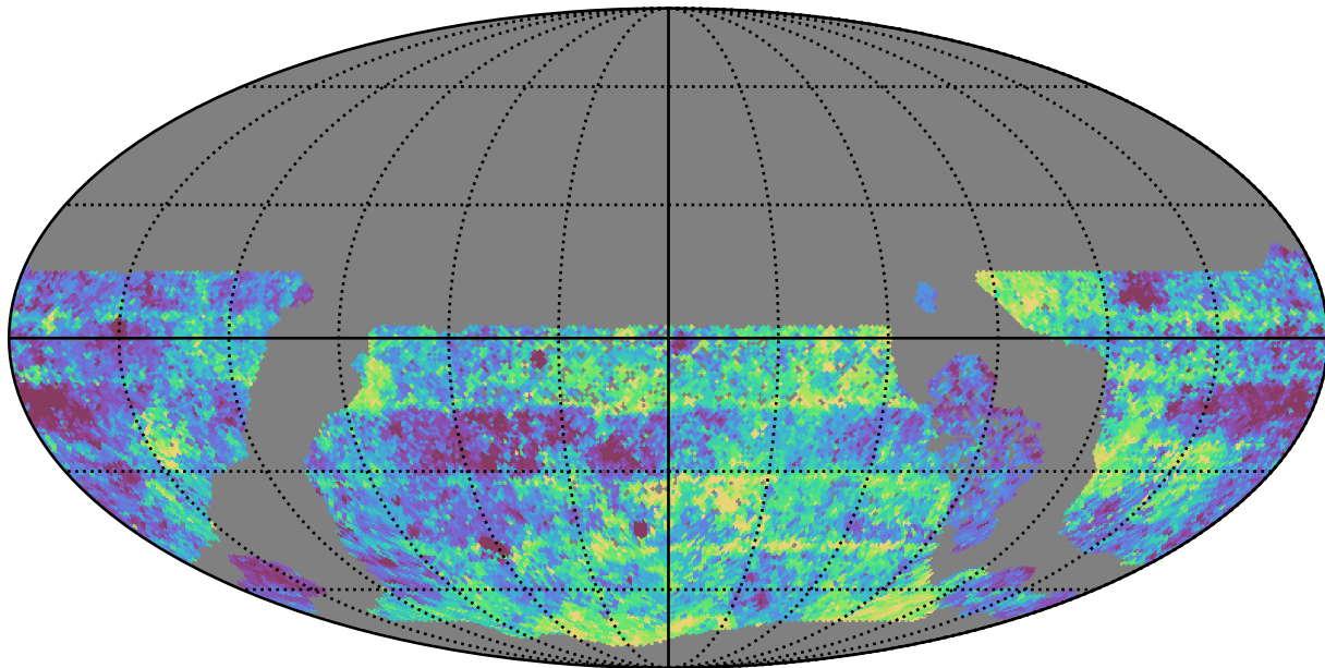
too_elab_r64_d2_giz_v3.4_10yrs WFD g band: Median Inter-Night Gap
