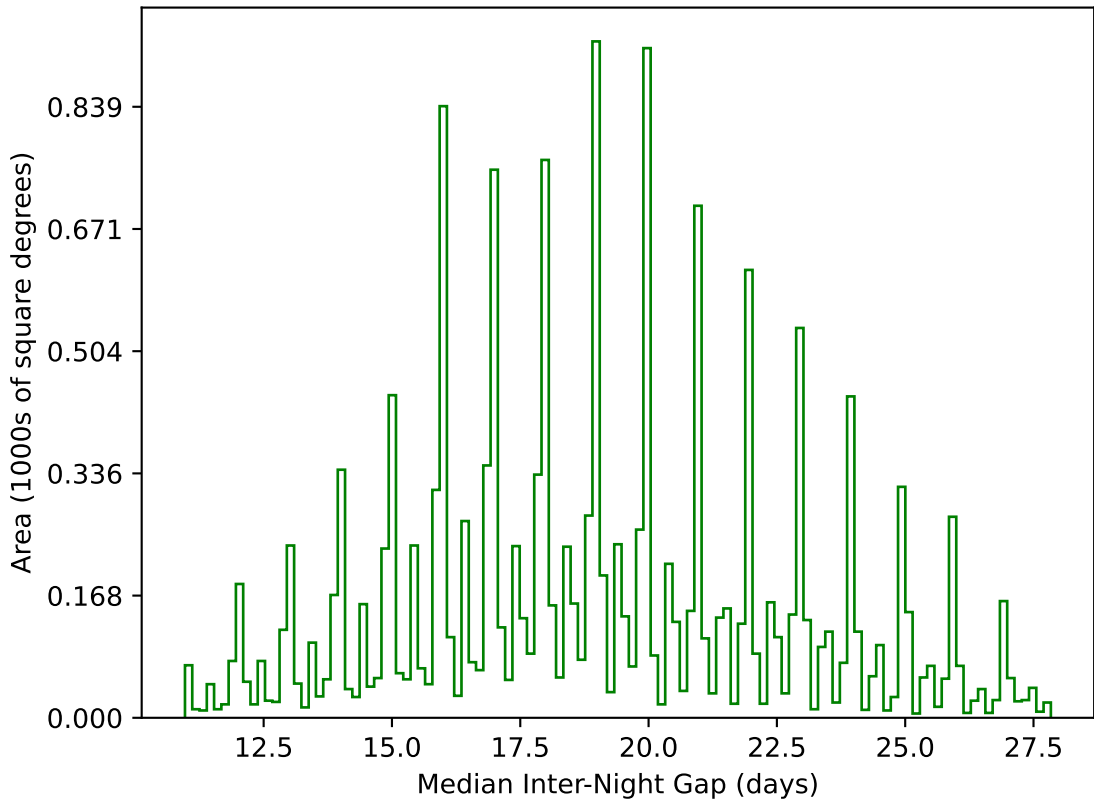
too_elab_r64_d2_giz_v3.4_10yrs WFD g band: Median Inter-Night Gap
