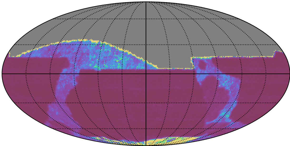
too_elab_r64_d2_giz_v3.4_10yrs All sky z band: Median Inter-Night Gap
