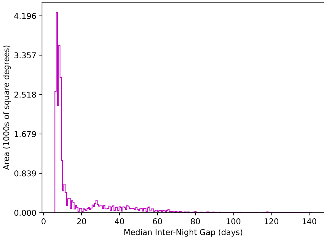
too_elab_r64_d2_giz_v3.4_10yrs All sky z band: Median Inter-Night Gap
