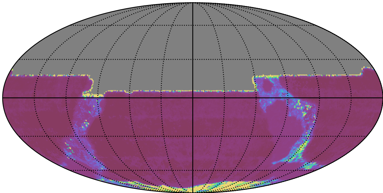
too_elab_r64_d2_giz_v3.4_10yrs All sky y band: Median Inter-Night Gap
