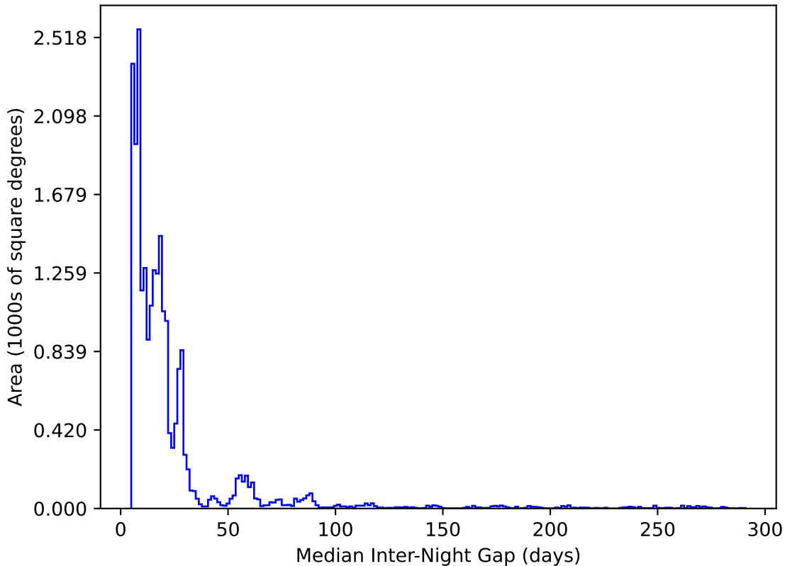
too_elab_r64_d2_giz_v3.4_10yrs All sky y band: Median Inter-Night Gap
