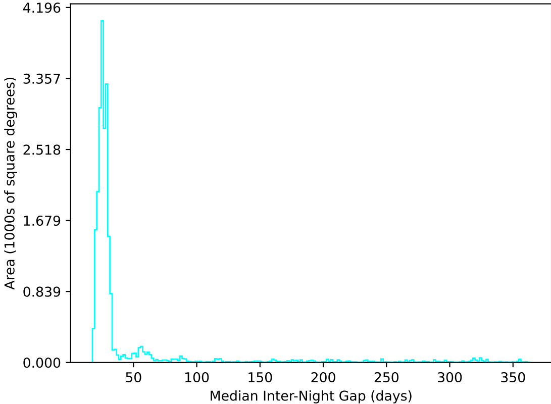
too_elab_r64_d2_giz_v3.4_10yrs All sky u band: Median Inter-Night Gap
