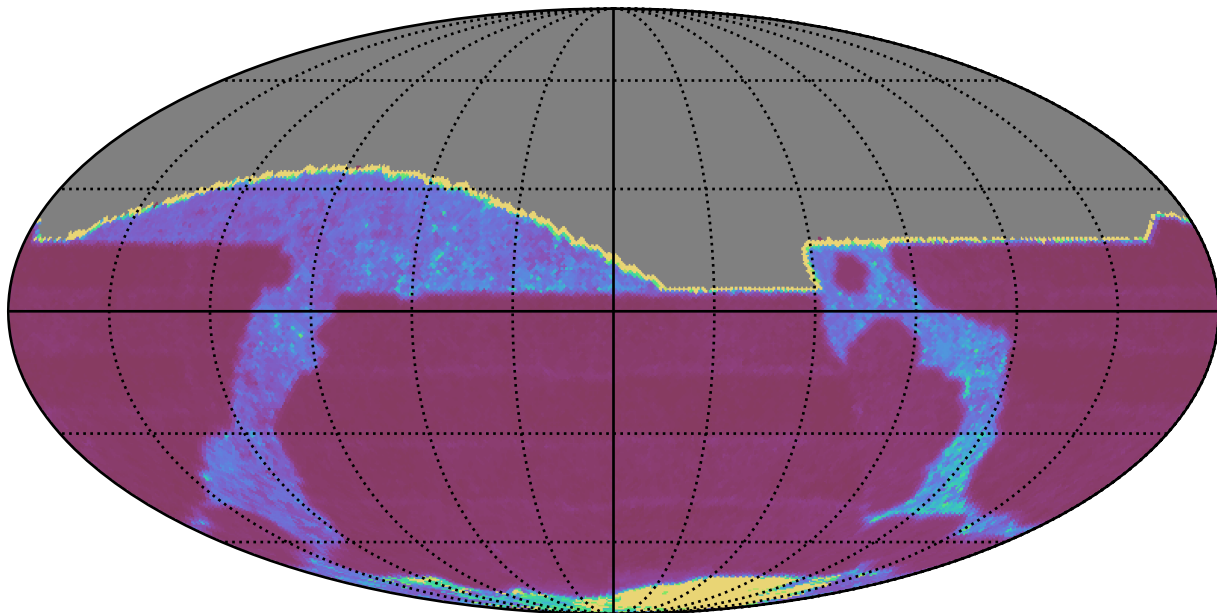
too_elab_r64_d2_giz_v3.4_10yrs All sky r band: Median Inter-Night Gap
