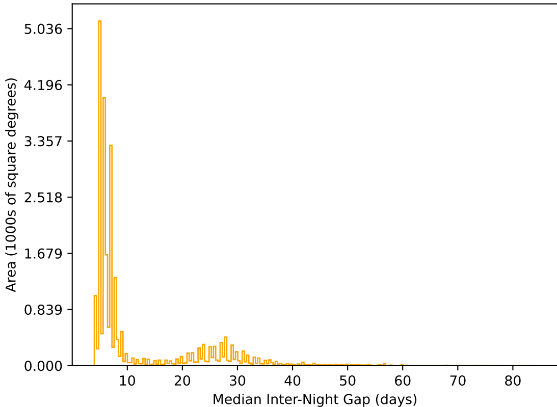
too_elab_r64_d2_giz_v3.4_10yrs All sky r band: Median Inter-Night Gap
