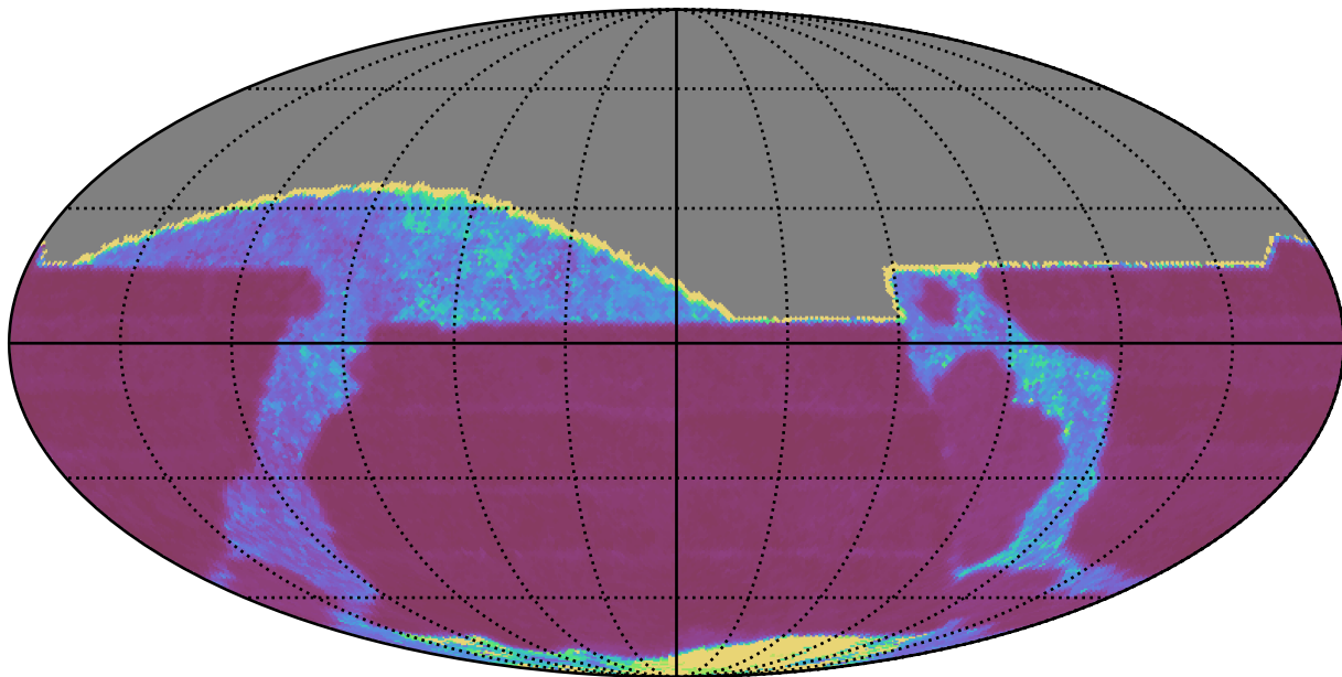
too_elab_r64_d2_giz_v3.4_10yrs All sky i band: Median Inter-Night Gap
