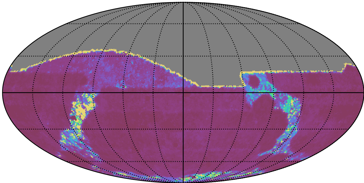
too_elab_r64_d2_giz_v3.4_10yrs All sky g band: Median Inter-Night Gap
