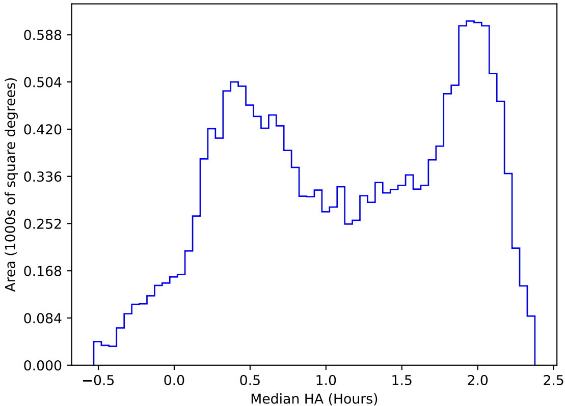
too_elab_r64_d2_giz_v3.4_10yrs WFD z band: Median HA
