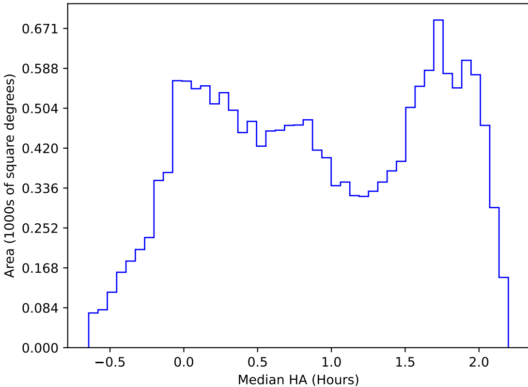
too_elab_r64_d2_giz_v3.4_10yrs WFD r band: Median HA
