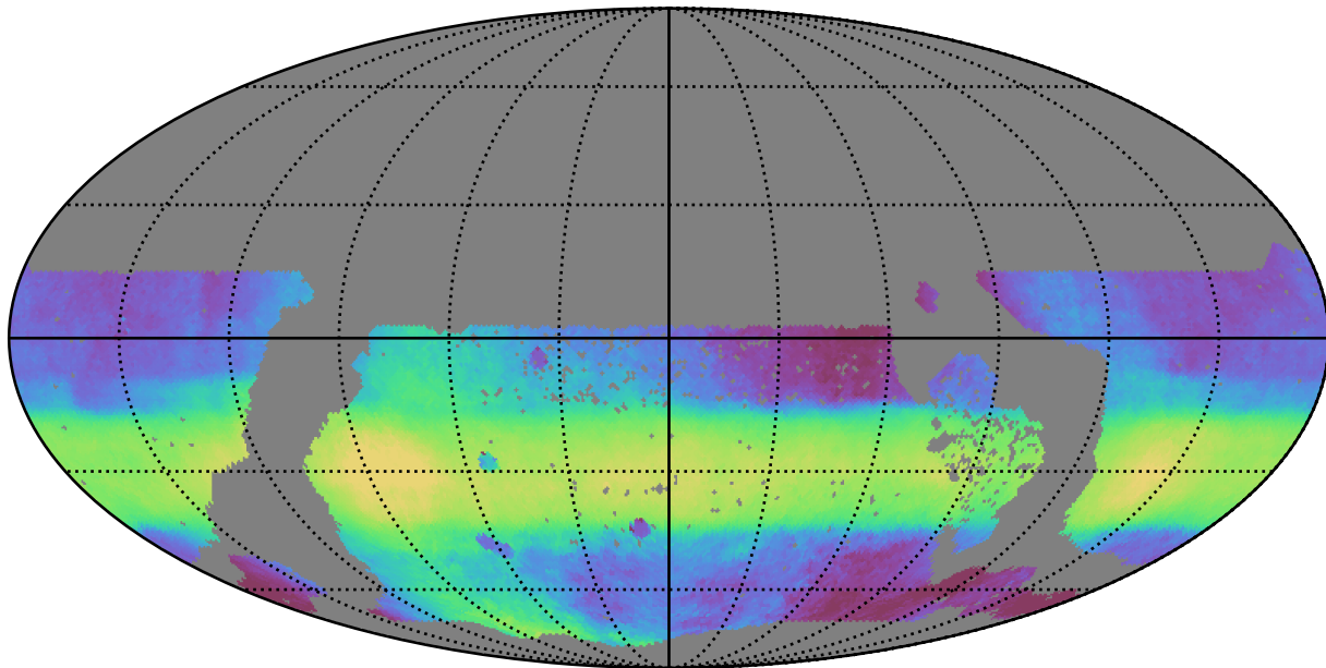
too_elab_r64_d2_giz_v3.4_10yrs WFD all bands: Median HA
