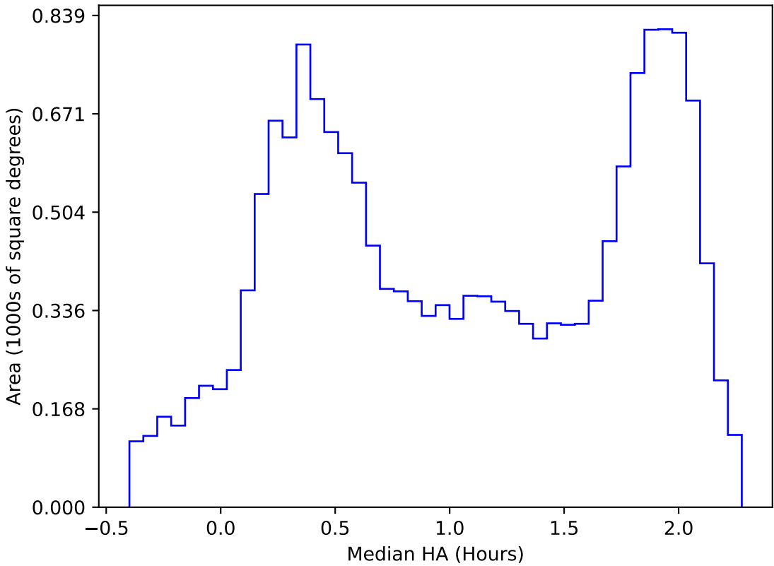
too_elab_r64_d2_giz_v3.4_10yrs WFD all bands: Median HA
