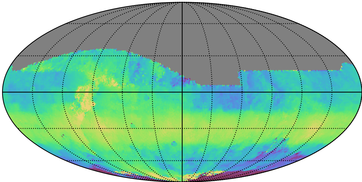
too_elab_r64_d2_giz_v3.4_10yrs All sky z band: Median HA
