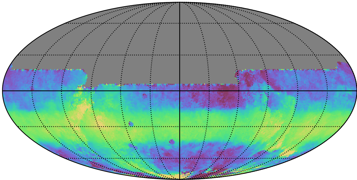
too_elab_r64_d2_giz_v3.4_10yrs All sky y band: Median HA
