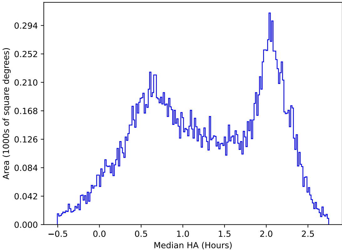
too_elab_r64_d2_giz_v3.4_10yrs All sky y band: Median HA
