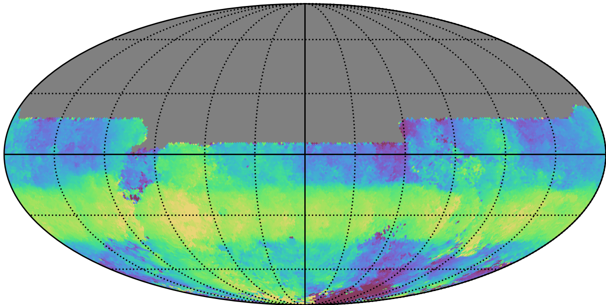
too_elab_r64_d2_giz_v3.4_10yrs All sky u band: Median HA
