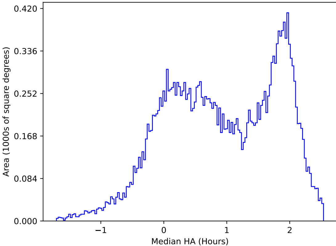
too_elab_r64_d2_giz_v3.4_10yrs All sky u band: Median HA
