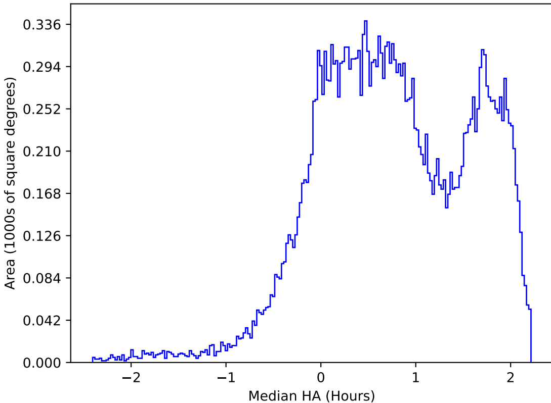
too_elab_r64_d2_giz_v3.4_10yrs All sky r band: Median HA
