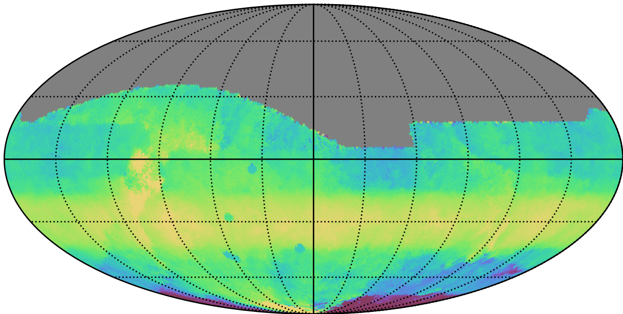
too_elab_r64_d2_giz_v3.4_10yrs All sky i band: Median HA
