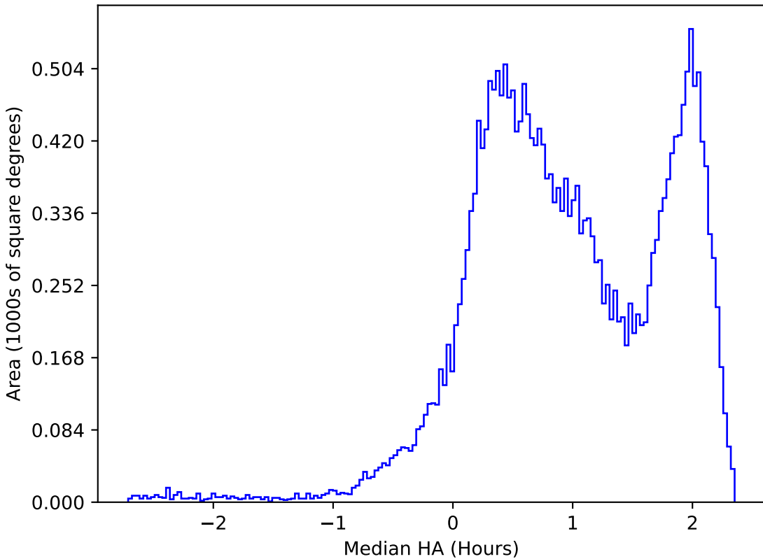
too_elab_r64_d2_giz_v3.4_10yrs All sky i band: Median HA
