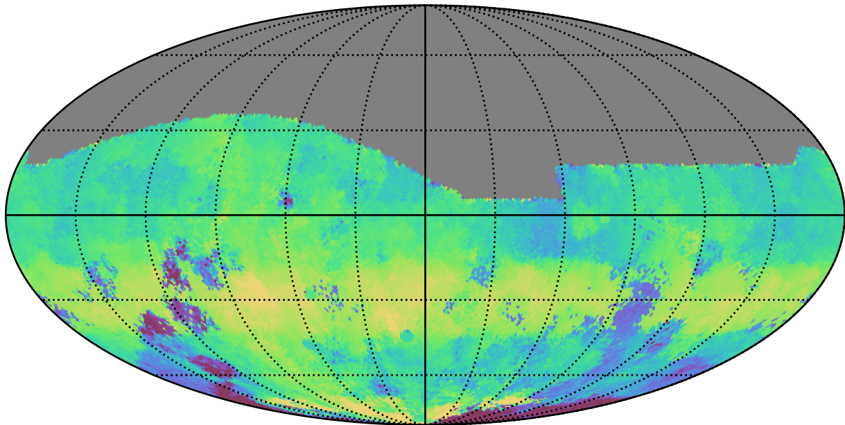
too_elab_r64_d2_giz_v3.4_10yrs All sky g band: Median HA
